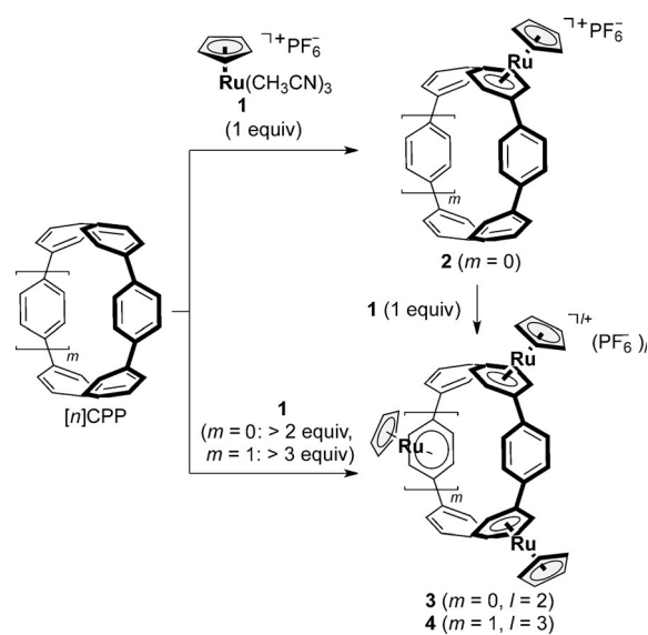
Scheme 1. Synthesis of mono- and multinuclear ruthenium [5] CPP and [6] CPP complexes.
